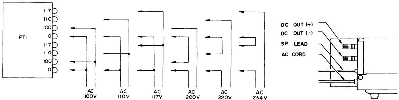
POWER TRANSFORMER PRIMARY CONNECTION
